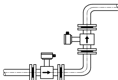
Fig. 9 - Vertical installation
