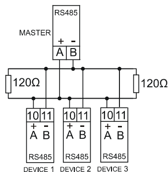
Fig. RS485 network connection peaters. Stations are connected to the link in parallel. The most distant ends of line have to be equipped with terminating resistors 120 Ω.
